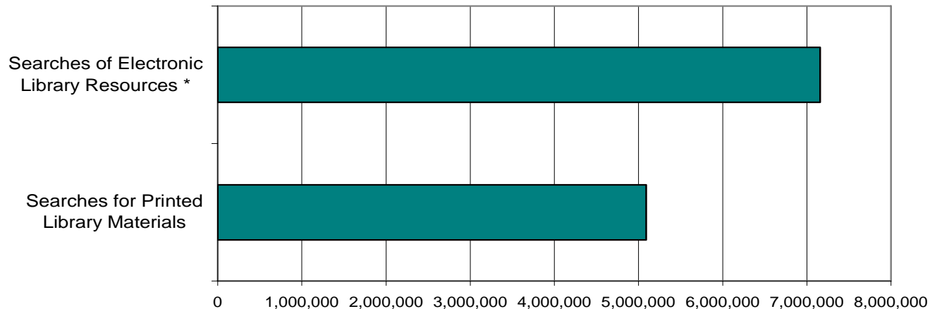
2005-06 Service Utilization
